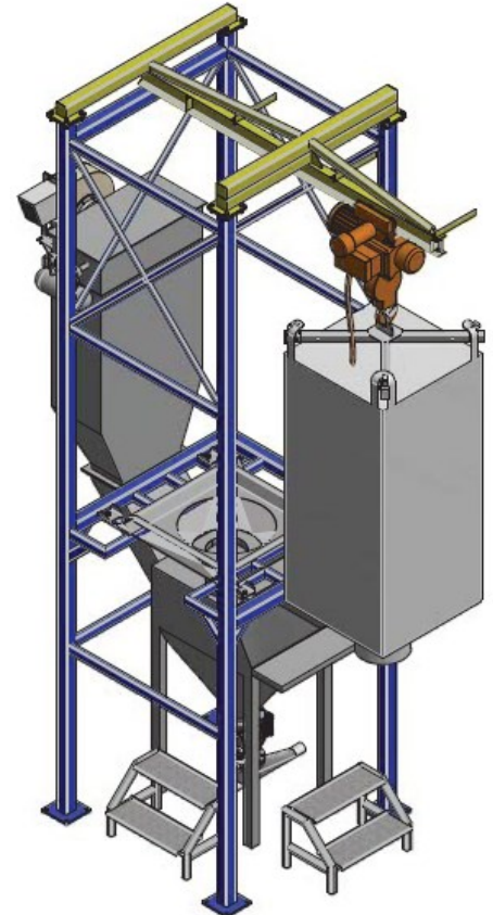
Bag & Bin Unloading Station
