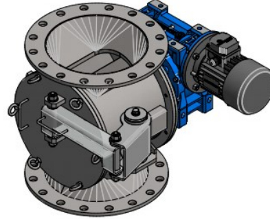
Air Lock Rotary Valve, Compact Type, Easy Clean Series
