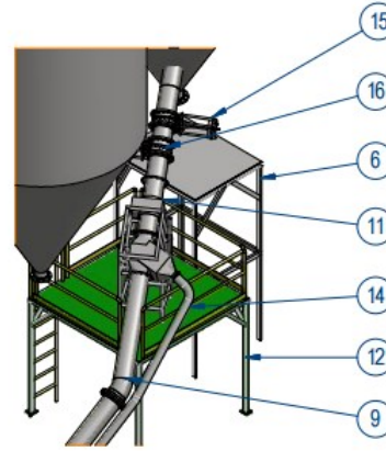
Metal Detecting System
