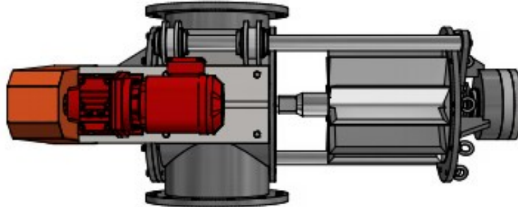
Air Lock Rotary Valve, Heavy Duty Slide Arm Type, Easy Clean Series
