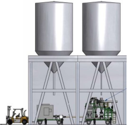
Mobile Sea Bulk Loading System
