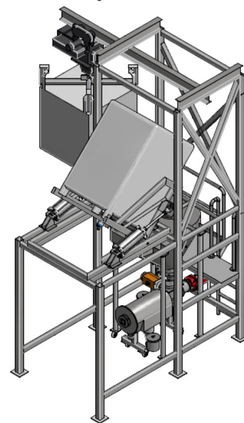
Bag & Bin Unloading Station
