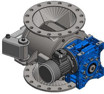
Air Lock Rotary Valve, Compact Type, Easy Clean Series
