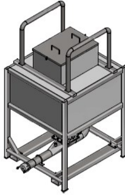
Dumping Bin
