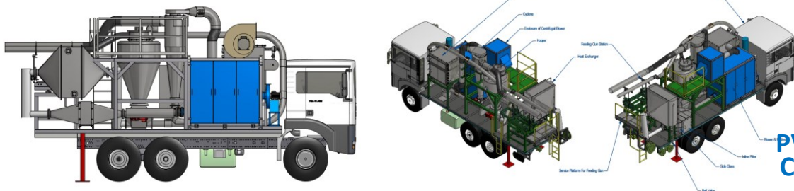
16 Tons/hour PE&PP Pellet Sea Bulk Container Mobile Loading Station
