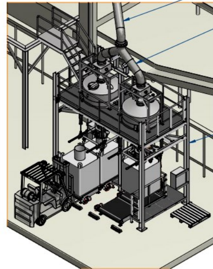
High Accuracy Automatic weighing System
