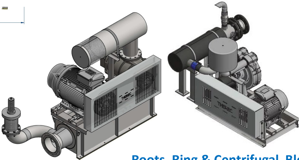
Roots, Ring & Centrifugal Blowers
