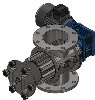
Air Lock Rotary Valve, Compact Type, Easy Clean Series
