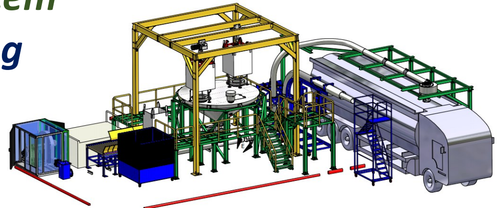
25 Tons/hour PE Pellet Sea Bulk Container & Bulk Truck Loading Station
