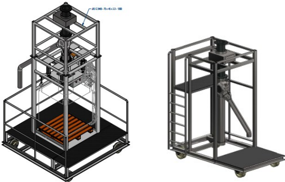
Mobile Big Bag filing Station & Mobile Metal Detector
