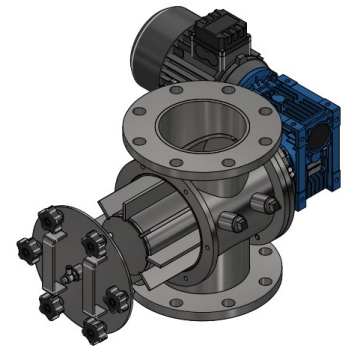
Air Lock Rotary Valve, Compact Dosing & Weighting Type, Easy Clean Series
