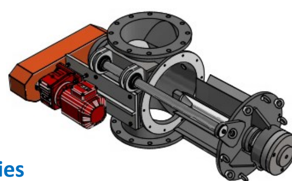
Air Lock Rotary Valve, Compact Dosing & Weighting Type, Easy Clean Series
