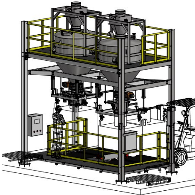
High Accuracy Automatic weighing System
