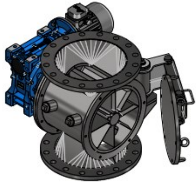
Air Lock Rotary Valve, Compact Type, Easy Clean Series
